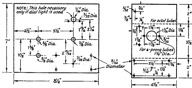
FIG. 2—DETAILS OF PANEL AND CHASSIS
