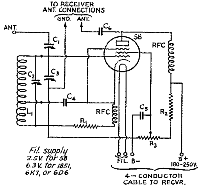
FIG. 1—CIRCUIT DIAGRAM OF THE PRESELECTOR WITH 5B TUBE IN USE
