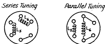
COIL FORM CONNECTIONS BOTTOM VIEW
