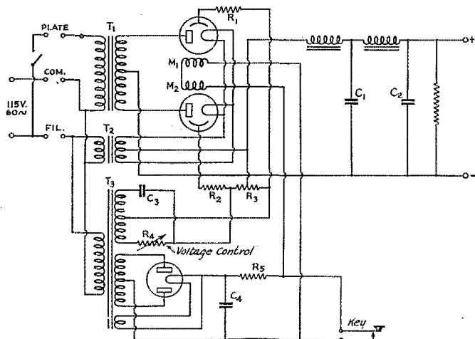
FIG. 2—PERMATRON POWER SUPPLY WITH VOLTAGE CONTROL T_1 —Plate transformer, 2500 volts, center-tapped. T_2 —Filament transformer, 2.5 volts, 10-amp. Secondary insulated for full plate voltage. T_3 —Control transformer, three secondaries: 300 volts center-tapped for voltage control; 500 volts for plates of 83 rectifier; 5 volts for 83 rectifier filament. M_1 , M_2 —Electro magnets. See text. R_1 , R_2 —100,000 ohms, 1-watt (for limiting grid current). R_3 —10,000 ohms, 25-watt wire-wound center-tapped. R_4 —2500 ohms, 25-watt variable. R_5 —4000 ohms, 75-watt. C_1 , C_2 —4- \mu fd., 1500-volt. C_3 —4- \mu fd., 1000-volt. C_4 —8- \mu fd., 600-volt electrolytic. Filter chokes and bleeder according to output current. See Handbook.
