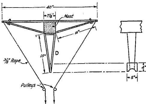
FIG. 7—ROTATING MECHANISM
