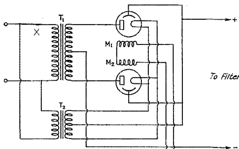
FIG. 1—MAGNETIC KEYING CIRCUIT FOR PERMATRONS R —4000 ohms, 75-watt. M_1 , M_2 —See text. T_1 —Plate transformer. T_2 —Rectifier filament transformer. X —Switch to allow preheating filaments.
